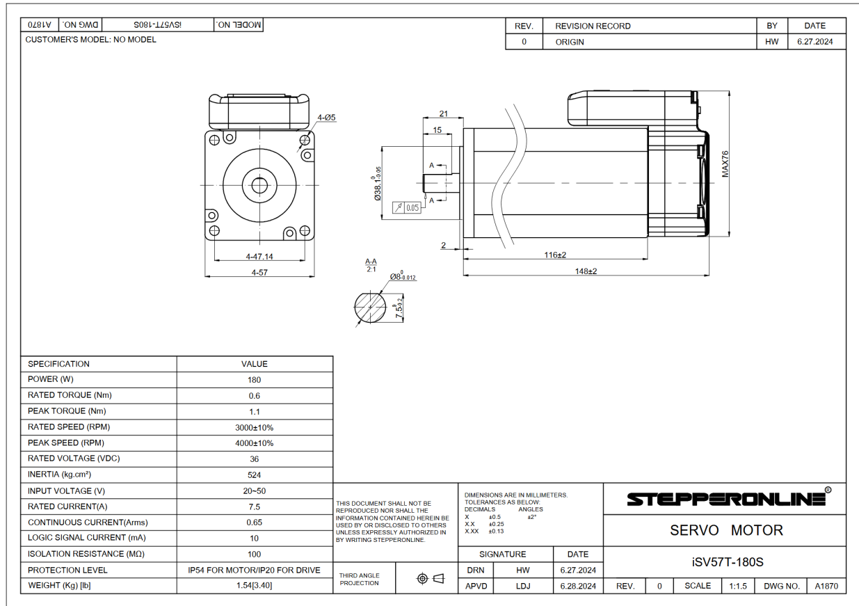
Figure 3. Selected motor data sheet.
